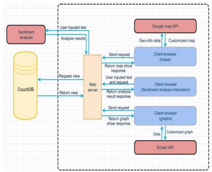
Fig 3.1: System Architecture of Web Application for Home Services
